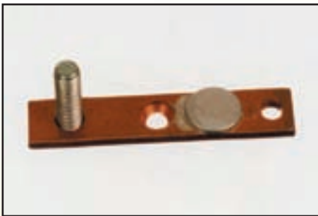
Description: HB 200 Amp Busbar (Single Stud - 13mm Tip)
