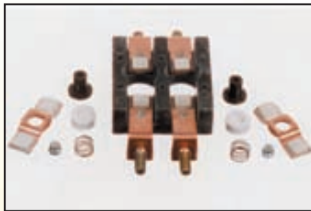
Description: HB Contact Kit (HB407 - 10mm Tip)
