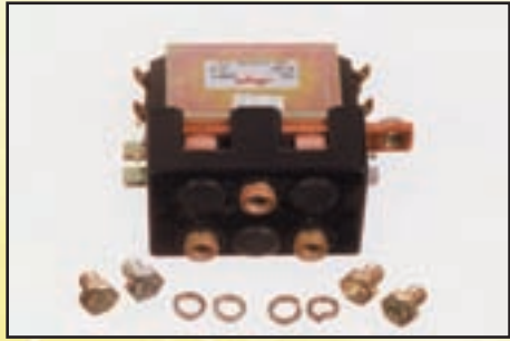
Description: Albright DC88 24 Volt Contactor
