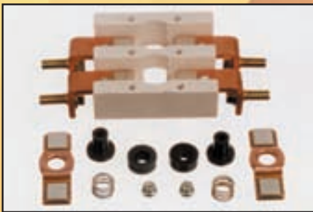
Description: HB Contact Kit (HB437 -10 Tip)
