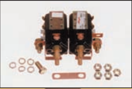
Description: Albright SW88 24 Volt Contactor
