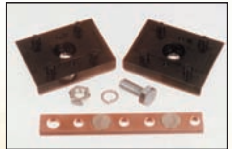
Description: Albright SW202 Fixed Back Contact (18mm Tip)
