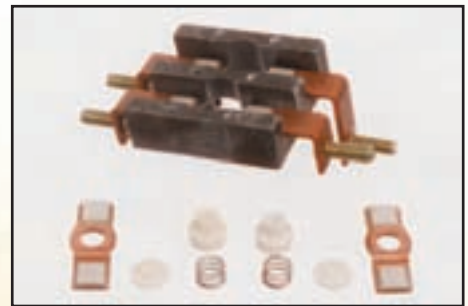
Description: HB Contact Kit (399707 & 925801 - 10mm Tip)
