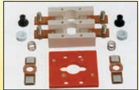
Description: HB Contact Kit (HB 437 - 10mm Tip)
