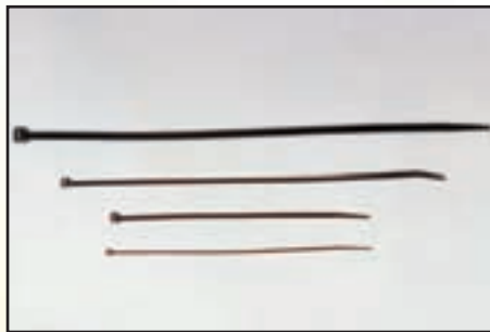
PART NO: 0-002-54 DESCRIPTION: 200 X 2.5MM CABLE TIES 1117B 200 X 4.8MM CABLE TIES 1119B 290 X 4.88MM CABLE TIES 1124B 370 X 7.6MM CABLE TIES 1127B 710 X 9.0 MM CABLE TIES
