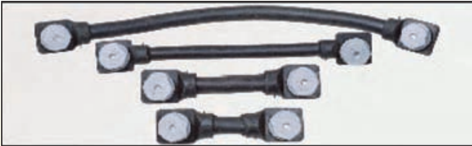
Description: Cable size from 16mm to 50mm available (State Length of Connector Required) We can also manufacture cable and harness assemblies to suit all applications.
