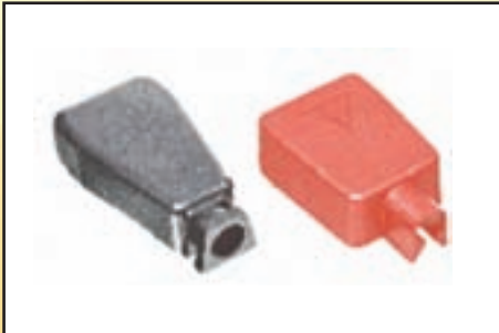
Description: 430 Series: Cable Entry - 17.3mm Length - 93.5mm Height - 23.4mm 417 Series: Cable Entry - 12.7mm Length - 80.2mm Height - 23.1mm
