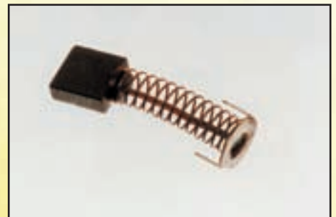
Description: Motor Brush Single Tail plus Spring 19 x 8 x 19mm
