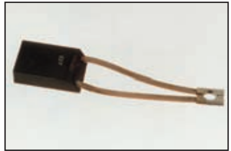
Description: Motor Brush Double Tail 25 x 12.5 x 40mm
