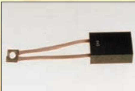
Description: Motor Brush Double Tail 25.5 x 14 x 35mm
