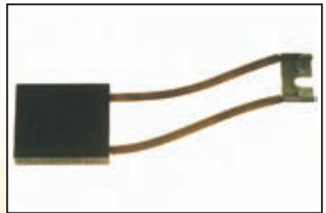
Description: Motor Brush Double Tail 40 x 12.5 x 46mm
