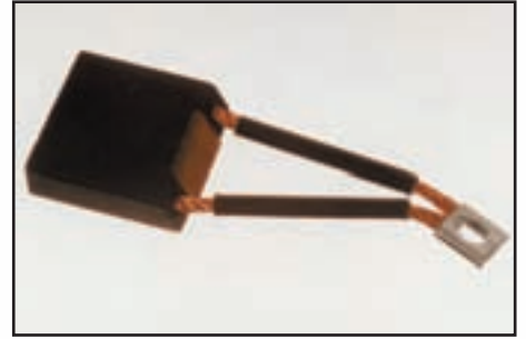
Description: Motor Brush Double Tail 40 x 12.5 x 40mm
