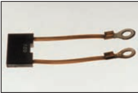
Description: Motor Brush Double Tail 27 x 6 x 19mm
