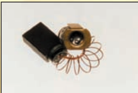
Description: Motor Brush Single Tail plus Spring 12.5 x 6 x 19mm
