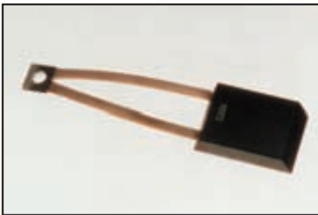
Description: Motor Brush Double Tail 25 x 10 x 35mm
