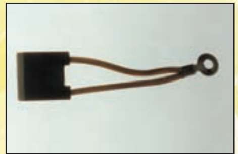
Description: Motor Brush Double Tail 25 x 11 x 25mm
