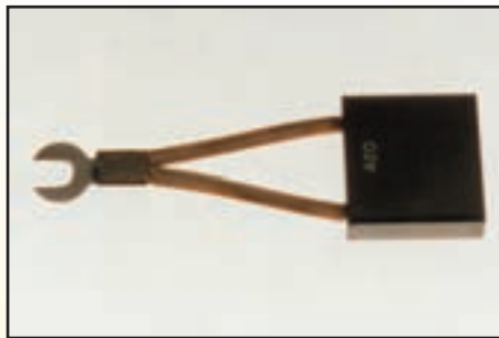
Description: Motor Brush Double Tail 31.5 x 9.5 x 28mm
