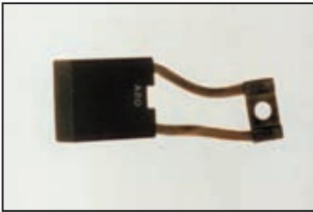
Description: Motor Brush Double Tail 25.5 x 11 x 30mm
