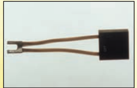
Description: Motor Brush Double Tail 31.5 x 12.5 x 32mm
