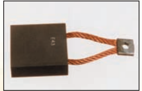
Description: Motor Brush Double Tail 12.4 x 31.6 x 32mm
