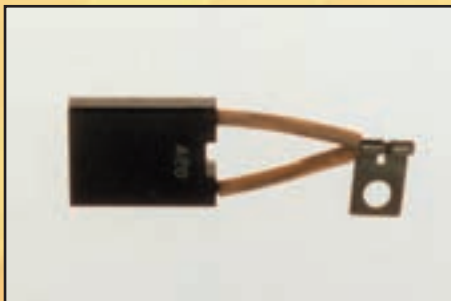
Description: Motor Brush Double Tail 22 x 6 x 28mm
