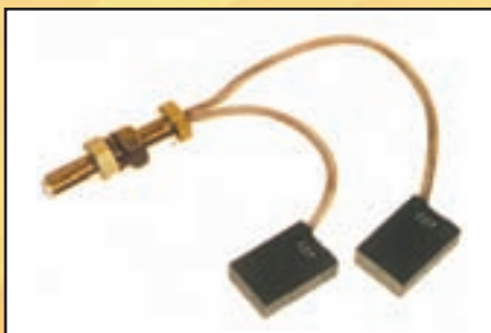
Description: Motor Brush Double Tail 17.5 x 8.5 x 25mm
