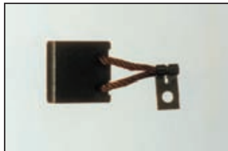
Description: Motor Brush Double Tail 26 x 9 x 26mm
