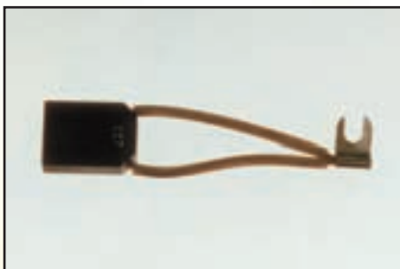
Description: Motor Brush Double Tail 19 x 9.5 x 25mm
