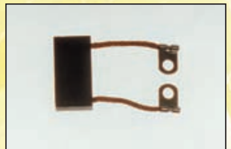
Description: Motor Brush Double Tail 38 x 9.5 x 19mm
